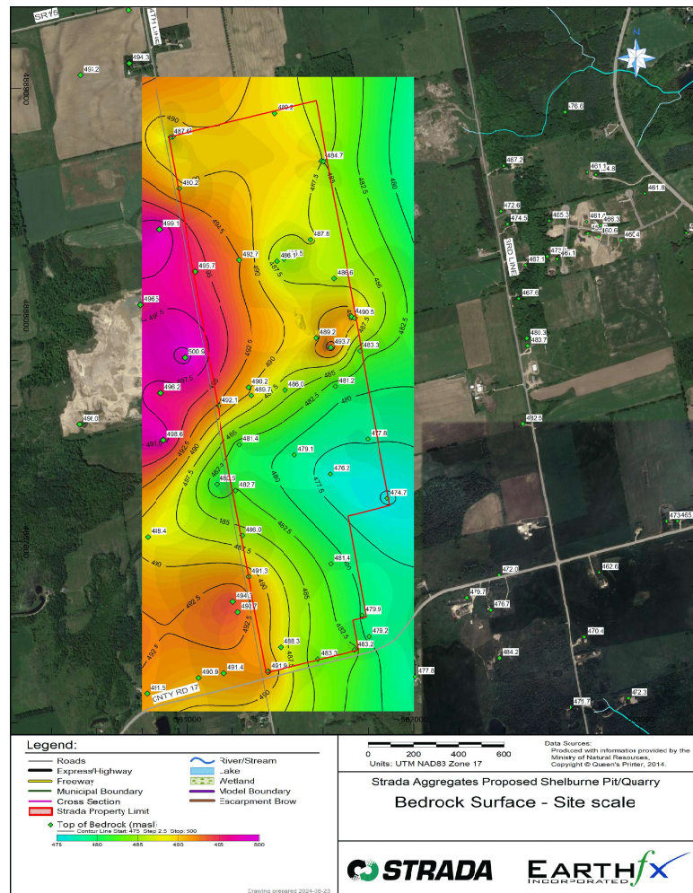
Figure 3.29: Bedrock Surface - Site Scale
