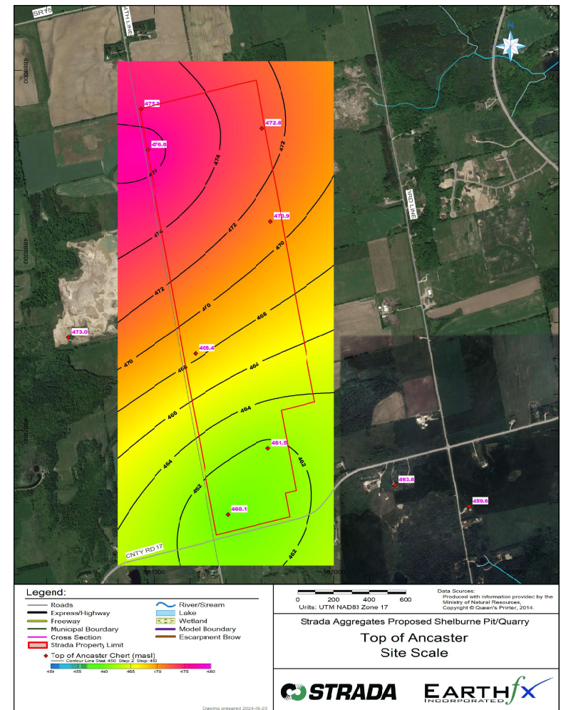
Figure 3.31: Top of Ancaster Member - Site Scale
